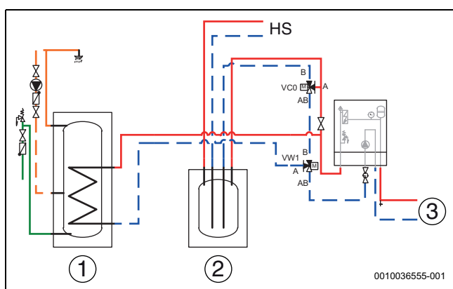
Fig. 28 Tampon, vanne bypass VCO
