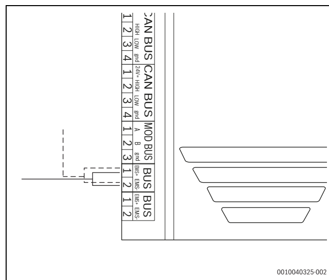
Afb. 48 Verbinding EMS
