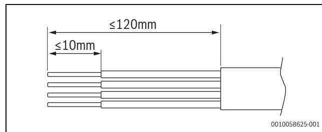
Afb. 47 Strippen CAN-BUS
