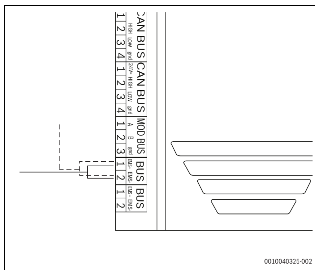
Afb. 50 Verbinding EMS
