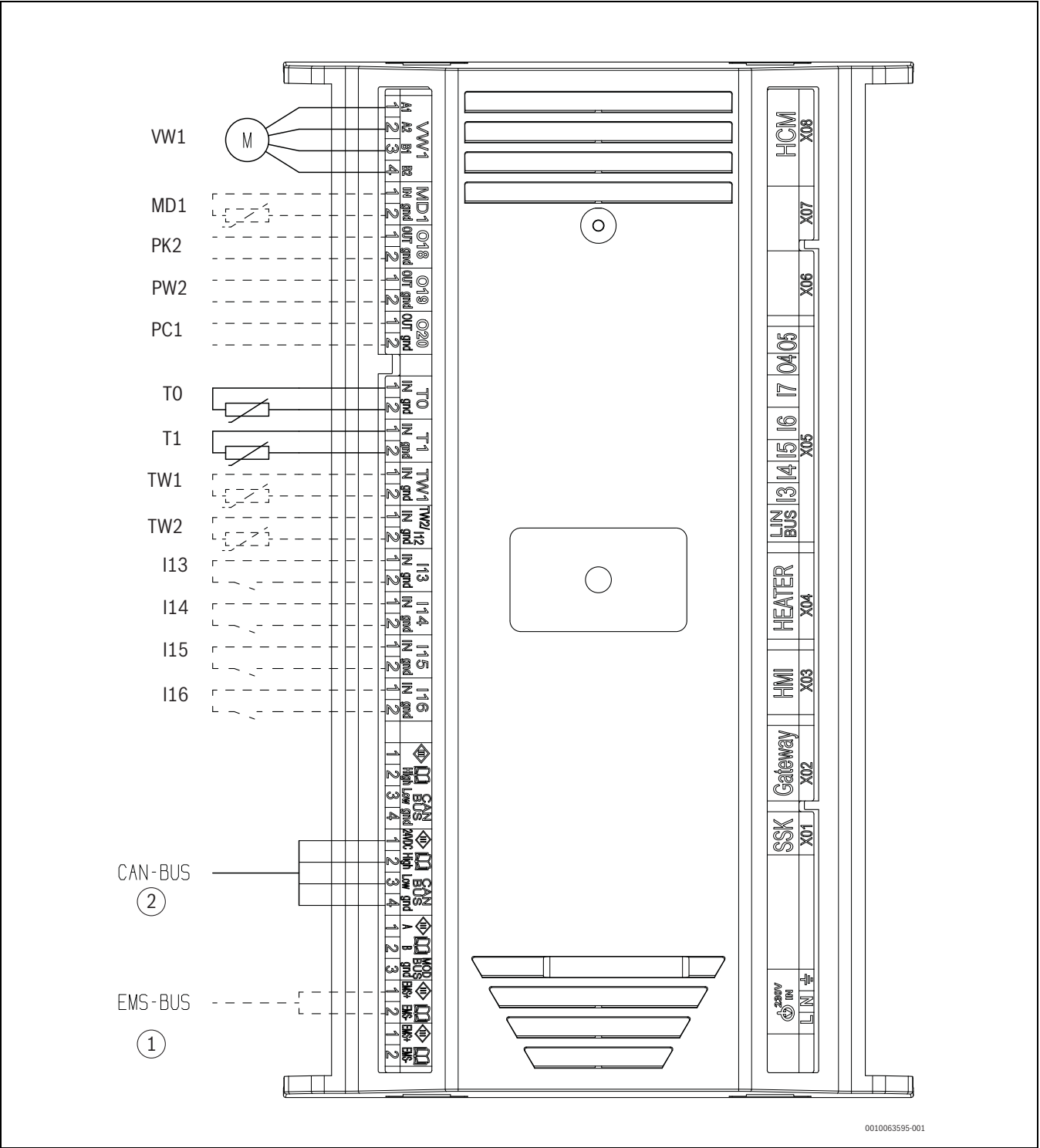
Fig. 46 XCU-THH de raccordement
