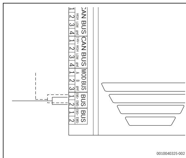
Fig. 50 Raccordement EMS
