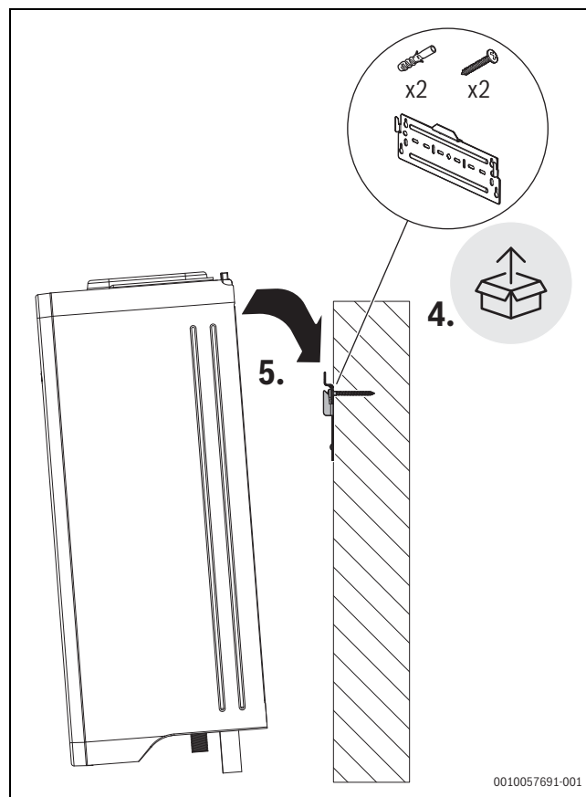
Fig. 10 Support mural
