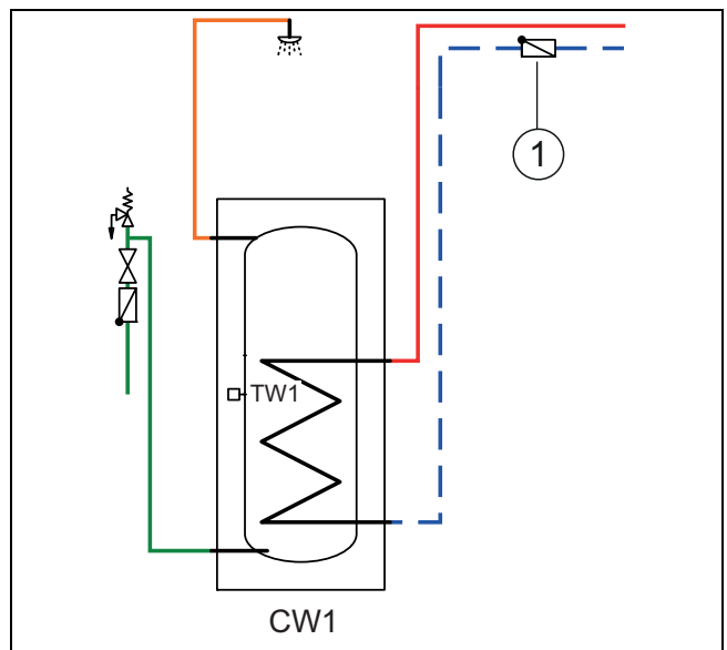
Afb. 19 Boiler
