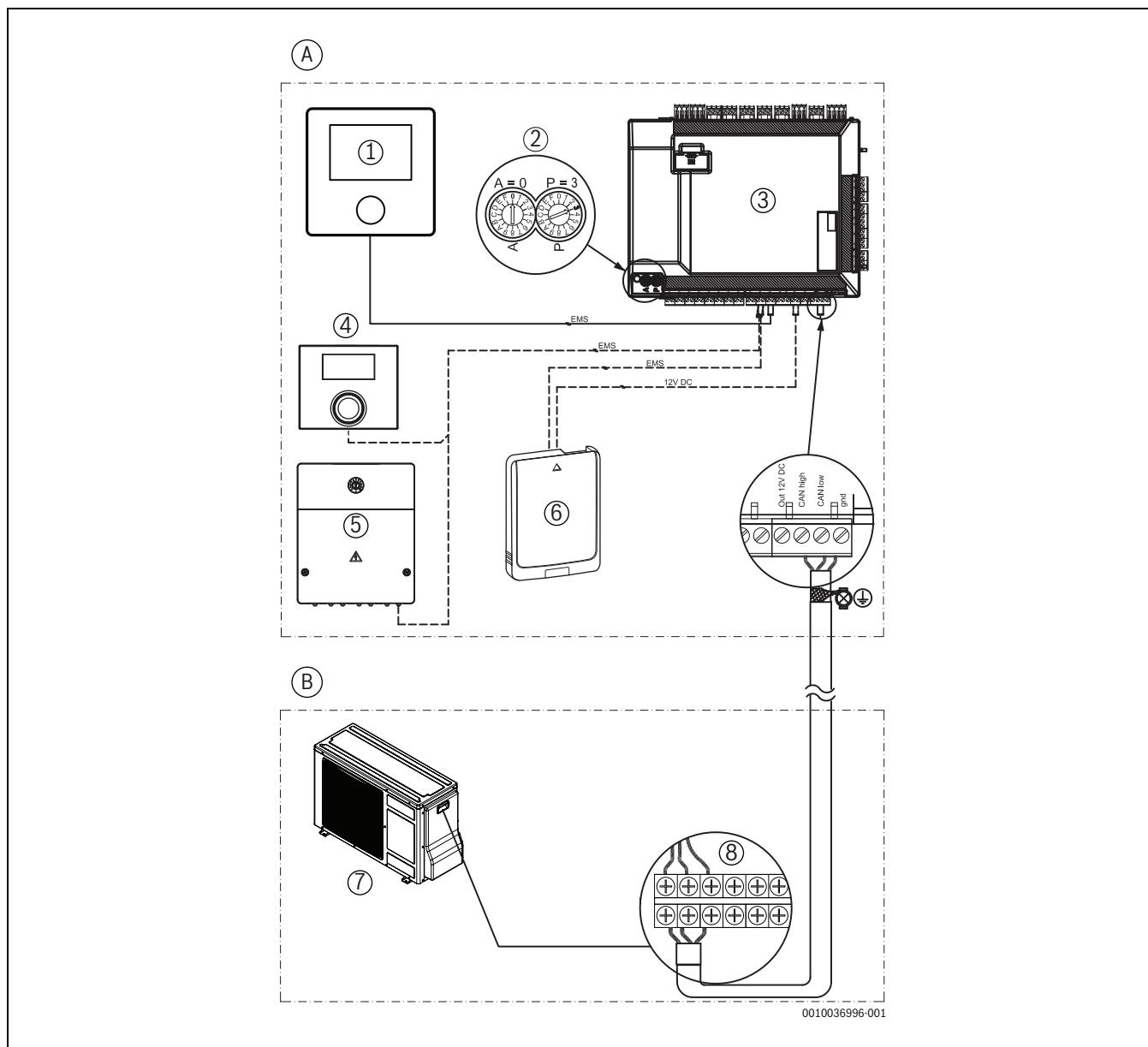
Fig. 41 Raccordements CAN et EMS
