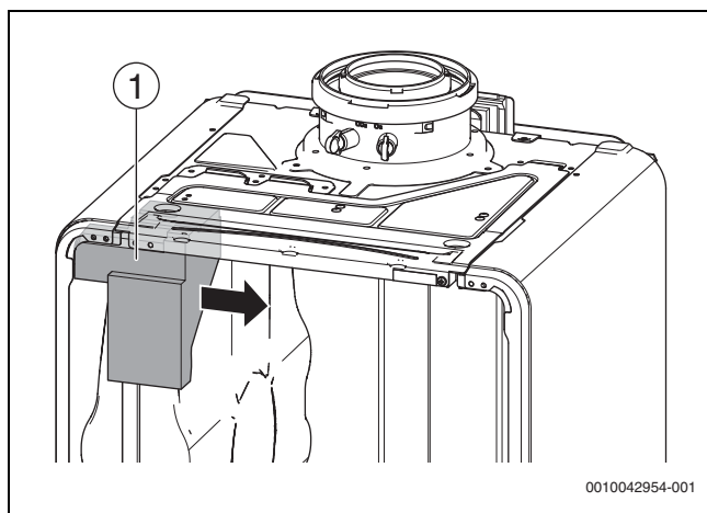
Fig. 29 Retirer la mousse de support
